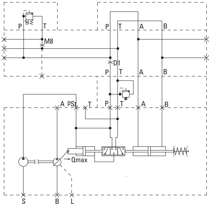
PVX Response Times DP - Control
