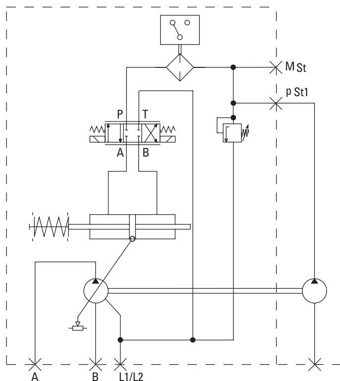
PVX RESPONSE TIMES SP - CONTROL
