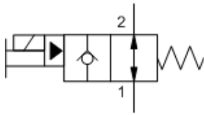
M-Control, H-Poppet
