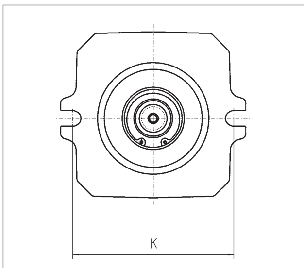
2-Loch Flansch
