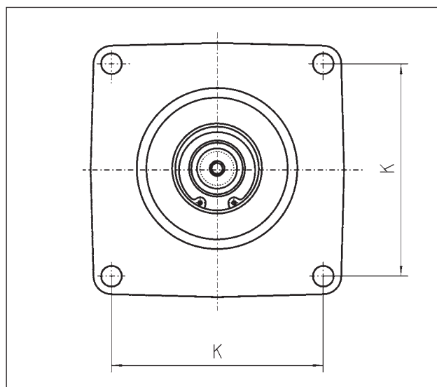
4-Loch Flansch
