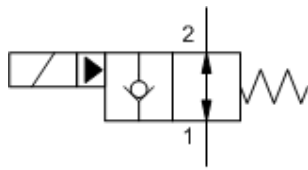
X-Control, H-Poppet
