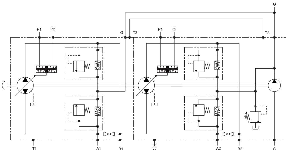
HYDRAULIC DIAGRAM
