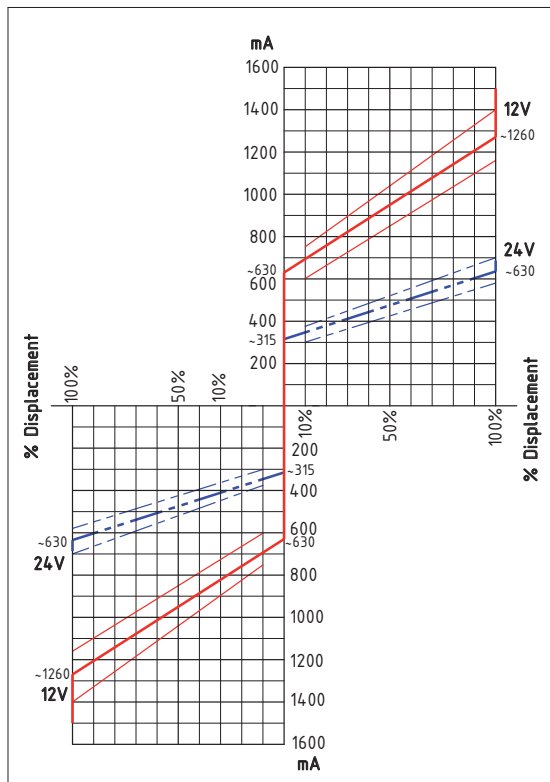
CURRENT-DISPLACEMENT GRAPHIC
