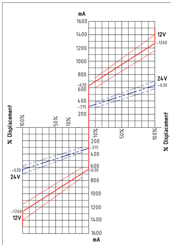
CURRENT-DISPLACEMENT GRAPHIC
