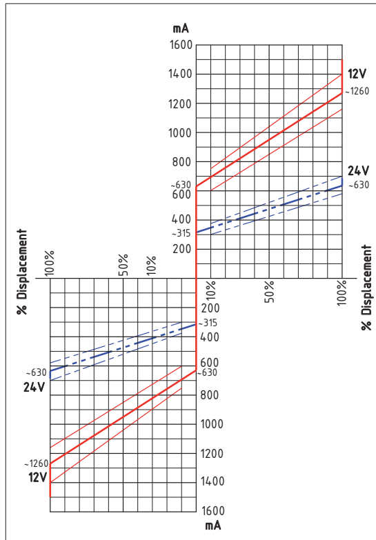
CURRENT-DISPLACEMENT GRAPHIC
