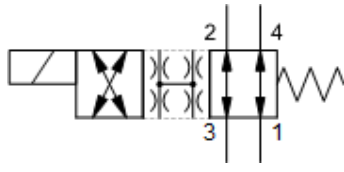
X-Control, N-Spool
