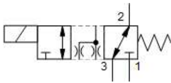
X-Control, N-Spool
