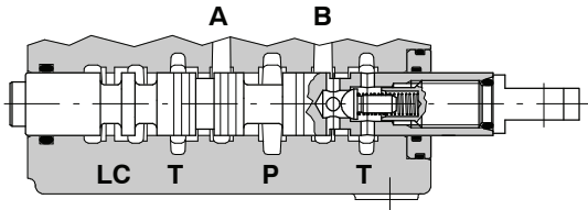
A-B→T (floating detent)
